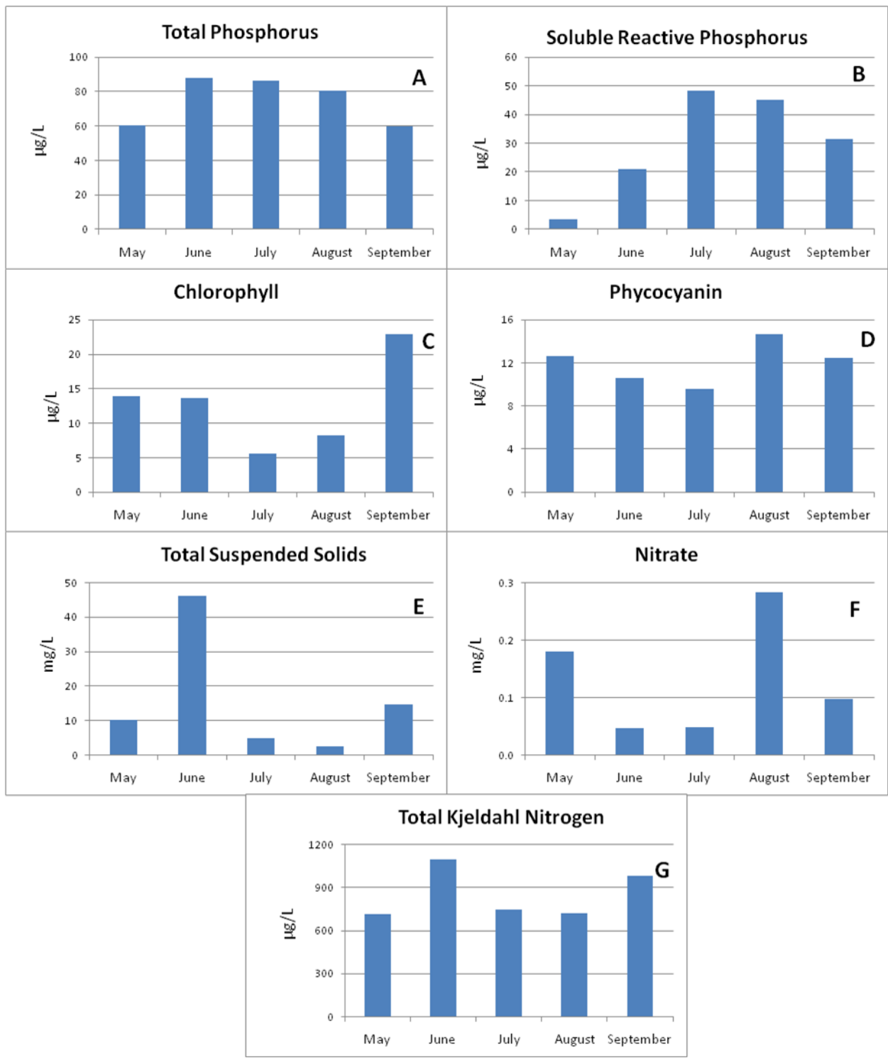
Figure 3. Average ( \pm S.E) seasonal concentrations of total phosphorus, soluble reactive phosphorus, chlorophyll a, phycocyanin, total suspended solids, nitrate, and total Kjeldahl nitrogen in Braddock Bay.
